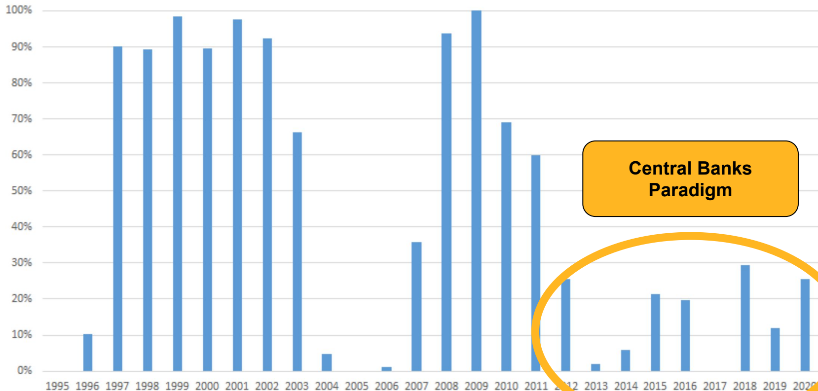
Proportion of days where VIX close is above average (average = 19)
